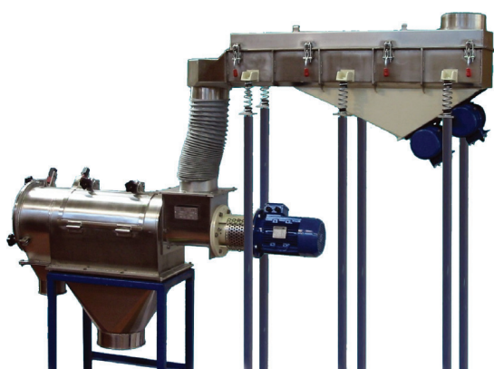
- Screening/refining unit
